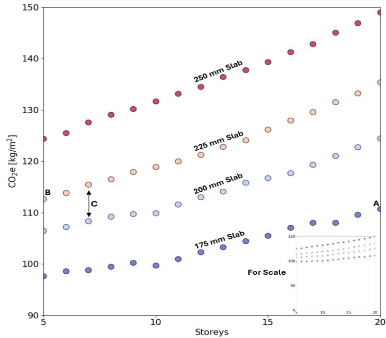
Figure 1: Global Warming Potential in CO 2 equivalents as the number of storeys increases for 4 different slab thicknesses.
